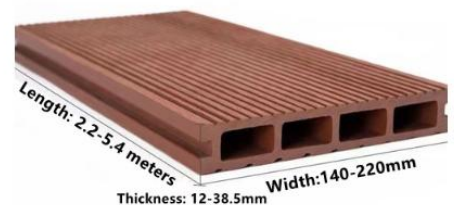
WPC Flooring Size (140-220mm)x(12-38.5mm)x(2.2-5.4m)
