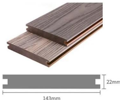
WPC Flooring size 143x22mm
